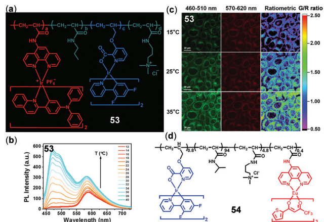
Fig. 38 (a) Chemical structure of copolymer 53 (a/b/c/d = 0.11/100/0.89/2.32). (b) Temperature-dependent emission spectra of 53 (0.01 w/v%) in PBS buffer (12–40 °C). (c) Confocal laser scanning microscopy images of HeLa cells labelled with 53 at 15 °C (top), 25 °C (middle), and 35 °C (bottom). Reprinted with permission from ref. 151. Copyright 2016 WILEY-VCH. (d) Chemical structure of copolymer 54 . Reprinted with permission from ref. 79. Copyright 2018 American Chemical Society.
