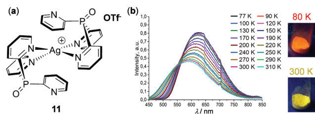
Fig. 10 (a) Molecular structure of Ag(I) complex 11 . (b) Normalized temperature-dependent emission spectral changes in the range of 77 – 310 \text{ K} . The pictures on the right show the solid emission colors of the samples at 80 and 300 \text{ K} , respectively. Reprinted with permission from ref. 77. Copyright 2019 the Partner Organisations.
