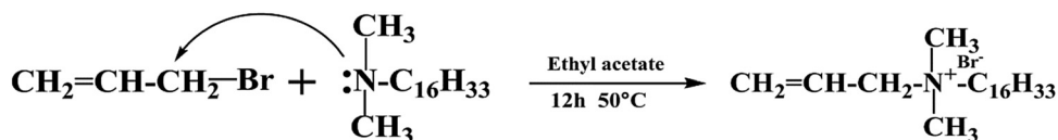
Fig. 2 Schematic representation of the preparation route of DMAHAB.
