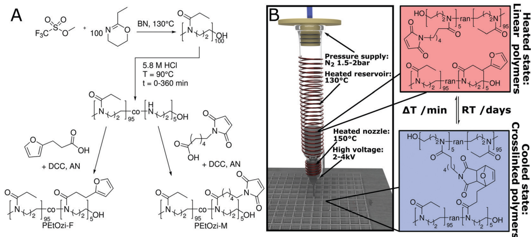
Fig. 1 (A) Synthesis of the furan and maleimide functionalized poly(2-ethyl-2-oxazine) (PETOzi-M, PETOzi-F) used in this study (DCC: dicyclohexyl carbodiimide, AN: acetonitrile, BN: benzoinitrile). (B) Schematic illustration of the MEW setup, processing conditions and the reversible DA equilibrium allowing liquefaction and melt processing at elevated temperatures followed by the chemically crosslinking upon cooling.
