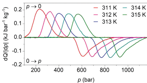
Fig. 4 Heat flow dQ/dp on applying ( 0 \rightarrow p ) and removing ( p \rightarrow 0 ) hydrostatic pressure, after baseline subtraction, at different temperatures.
