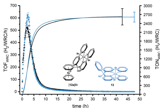
Fig. 4 Photocatalysis experiment with [12\text{a}]^+\text{Br}^- in black and the parent catalyst 13 in blue. TOF (dots) ( \text{H}_2/\text{Co}/\text{h} ) and TON (lines) ( \text{H}_2/\text{Co} ) formed as a function of time for 5 \mu\text{M} catalyst. Experimental conditions: 10 mL solution, 0.5 mM [\text{Ru}(\text{bpy})_3]\text{Cl}_2 , 0.1 M NaAsc, 0.1 M TCEP, pH 5.0, 453 nm LED irradiation.
