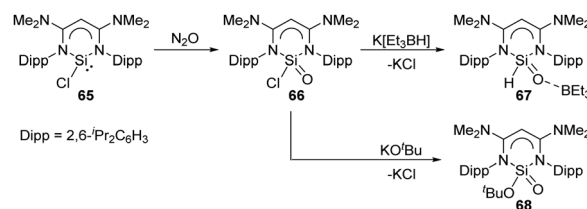
Scheme 25 Activation of N_2O by the chlorosilylene 65 and further metathesis reaction at the Si centre.
