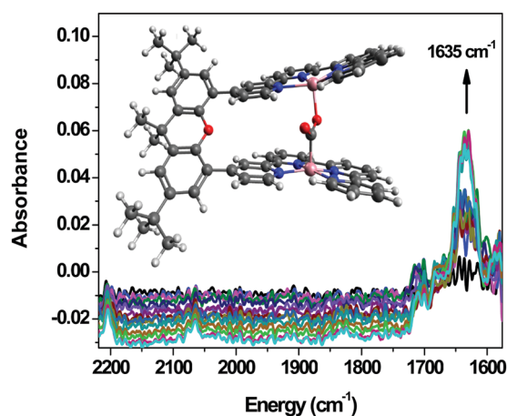
Fig. 14 Infrared spectro-electrochemistry data on a 1 mM solution of Co23 in \text{CH}_3\text{CN} (0.1 M t\text{Bu}_4\text{NPF}_6 , 0.5 M TEA) under \text{CO}_2 at potentials between -0.35 \text{ V} and -0.85 \text{ V} vs. Ag pseudo-reference. Inset: Calculated structure of the \text{CO}_2 -reduced complex adduct identified at 1635 \text{ cm}^{-1} . Adapted with permission from ref. 40. Copyright 2019, Springer Nature.
