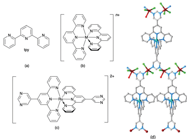
Fig. 1 (a) The structure of 2,2':6',2''-terpyridine (tpty) showing the trans , -trans conformation of the free ligand. (b) The \{M(tpty)_2\} -motif with the ligand in the cis,cis conformation adopted in the bis-chelate. (c) An example of an \{M(tpty)_2\} -centred expanded ligand, and (d) its use as a building block in a 2D-coordination network (CSD refcode BODGOR, with H atoms omitted).
