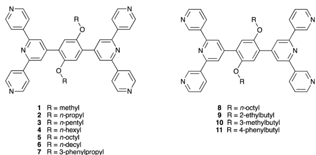
Scheme 4 Structures of tetatopic ligands with 4,2':6',4''\text{-tpy} domains (left) and 3,2':6',3''\text{-tpy} domains (right).
