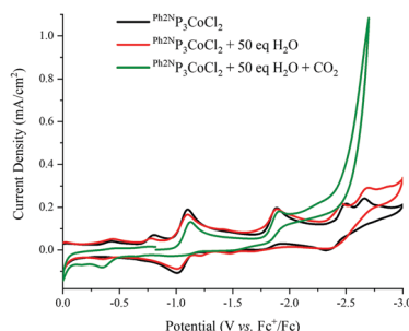
Fig. 3 Cyclic voltammograms of 1\text{ mM } [\text{Ph}^{\text{H}}\text{N}^{\text{H}}\text{P}_3\text{CoCl}_2] under various conditions. (Black): under \text{N}_2 ; (red): in the presence of 50 eq. \text{H}_2\text{O} ; (green): in the presence of 50 eq. \text{H}_2\text{O} and \text{CO}_2 . Conditions: GC working electrode, 0.1 M TBAPF 6 electrolyte in MeCN solvent, scan rate of 0.06\text{ V s}^{-1} , initial scan is positive.
