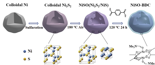
Scheme 5 Schematic illustration of the preparation of Ni-BDC-modified \text{Ni}_3\text{S}_2/\text{NiS} (NiSO-BDC) hollow nanoparticles. Reprinted with permission from (ref. 126). Copyright (2019) American Chemical Society.
