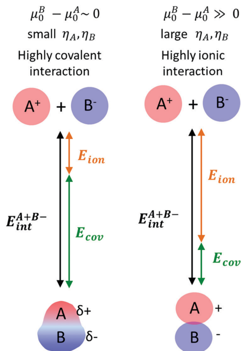
Scheme 7 Effects of chemical strength and hardness of species A and B on the nature of \text{A} + \text{B}^- ion-pair interaction.
