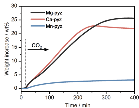
Fig. 2 Isothermal TGA profiles of M -pyz ( M = \text{Mg}^{2+}, \text{Ca}^{2+}, \text{Mn}^{2+} ) under \text{CO}_2 flow (0.1 MPa, 30\text{ mL min}^{-1} ) at 40^\circ\text{C} .
