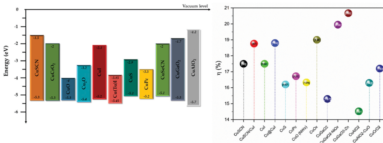
Fig. 26 Energy levels of the Cu-based materials discussed in this review (left) and graph of power conversion efficiencies for each material, with the corresponding reference number (right).
