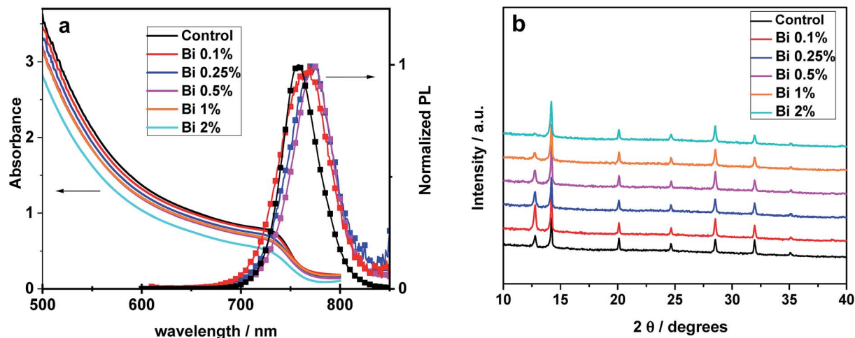
Fig. 2 Characterization of thin films with different Bi content on glass (a) absorption spectra, which are rather unaffected apart from a slight broadening of the onset. Normalized photoluminescence showing a slight red shift for higher Bi concentrations. (b) XRD data not showing any significant changes in the perovskite structure nor new phases.
