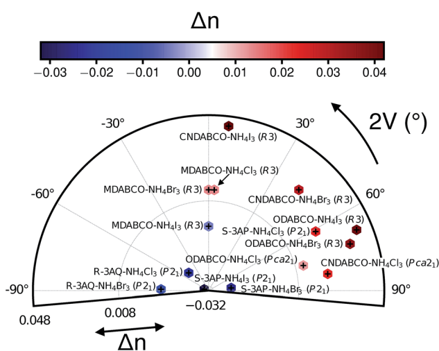
Fig. 2 Computed birefringence \Delta n and 2V angle of metal-free perovskites at their experimental volume and lattice constants. \Delta n is plotted on the radial axis and using the colour-bar, with red indicating positive \Delta n . Values of n are given in Table S3 of the ESI.† The 2V angles provide information about the nature of the birefringence in biaxial crystals.
