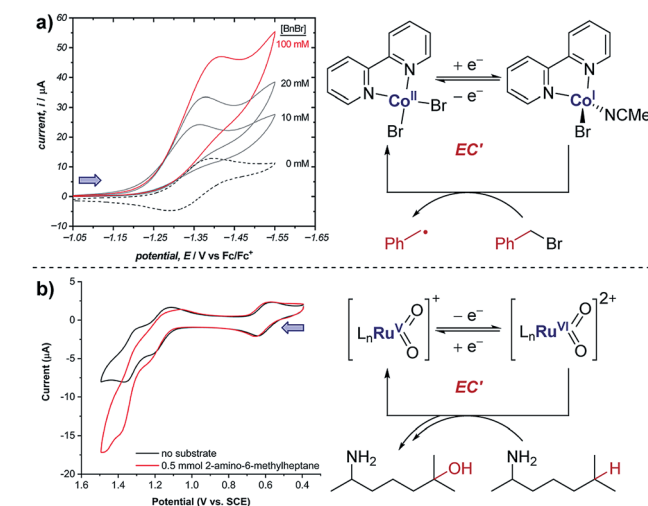
Fig. 7 (a) Evidence of electrocatalysis (EC' mechanism) by a ligated Co(II) species through oxidative addition of benzyl bromide, reported by the groups of Minter and Sigman. Blue arrow in figure demonstrates the direction of the scan, positive current represents reduction. Adapted with permission from ref. 20. Copyright 2019 American Chemical Society. (b) Determination of catalytic Ru oxidation states from the increase in current due to catalysis, reported by the groups of Du Bois, Waymouth, Sigman and Zare. Blue arrow in figure demonstrates the direction of the scan, positive current represents reduction. Adapted with permission from ref. 21. Copyright 2019 American Chemical Society.
