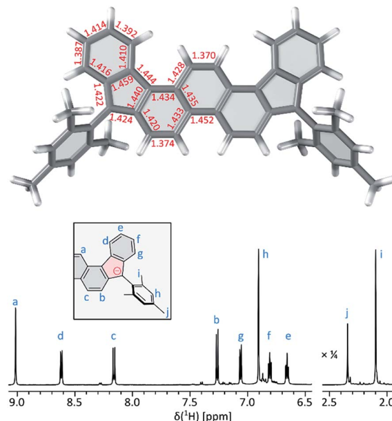
Fig. 5 ^1\text{H} NMR spectrum ( \text{THF-}d_8 , 600 MHz, 300 K, bottom) and DFT-optimized geometry of 2^{2-} (PCM( \text{THF} )/B3LYP/6-31G(d,p), top).
