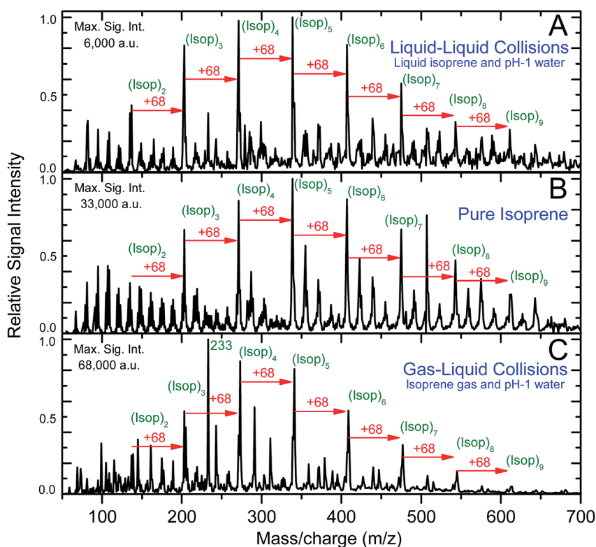
Fig. 2 ESIMS spectra for sets of experiments A, B, and C: the dominant peaks correspond to protonated oligomers of isoprene, [(Isop) n ·H] + , and the secondary peaks correspond to fragments of the isoprene molecules bonded to the primary oligomers. (A) ESIMS spectra of the organic phase from the emulsion of liquid isoprene in water at pH = 1 and air (1 : 6 : 3 v/v/v) that was agitated at 1200 rpm for 360 minutes. (B) ESIMS spectra of as-purchased liquid isoprene. (C) ESIMS spectra of products of gas–liquid collisions between water (pH = 1) and gas-phase isoprene (Methods).
