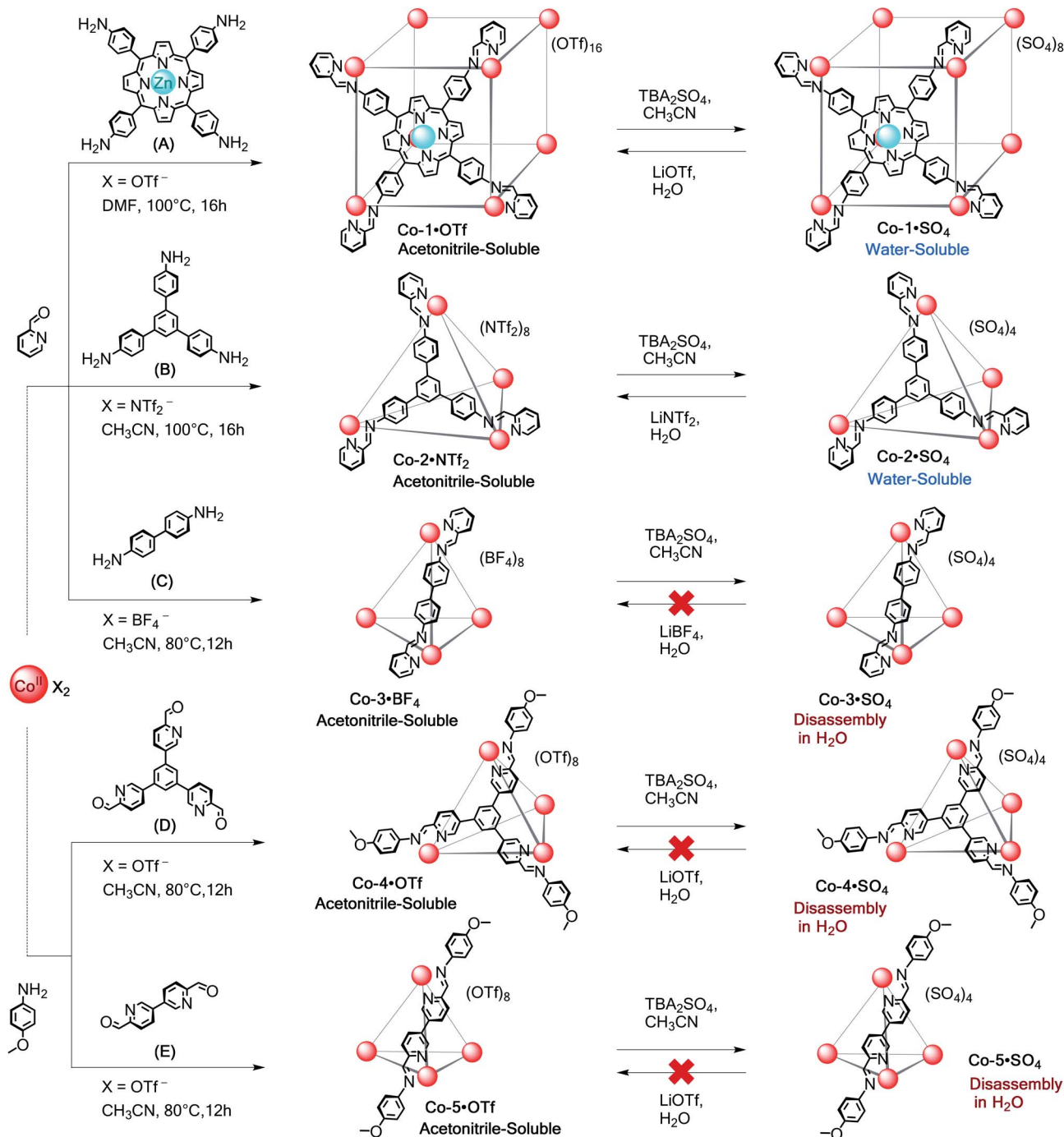
Scheme 1 Subcomponent self-assembly of \text{Co}^{\text{II}} -capsules. Preparation of acetonitrile-soluble Co-1 \cdot\text{X} to Co-5 \cdot\text{X} ( \text{X} = \text{OTf}^- , \text{NTf}_2^- , or \text{BF}_4^- ) from subcomponents A–E and their anion exchange sequences.
