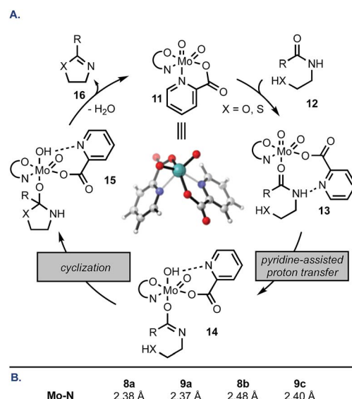
Scheme 1 (A) Proposed mechanism of Mo-catalysed cyclodehydration (second carboxylate ligand abbreviated for clarity). (B) Selected geometrical parameters of \text{MoO}_2(\text{X})_2 complexes optimized at B3LYP/6-31G(d)/LANL2DZ level of theory. The optimized structure of the thermodynamic complex of \text{MoO}_2(\text{pic})_2 , pic = 2-picolinate is presented in the middle of the catalytic cycle.
