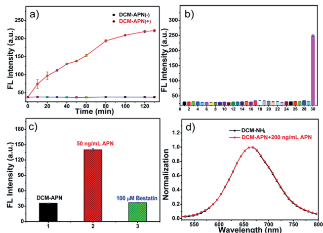
Fig. 2 (a) Time response of probe DCM-APN versus APN. (b) Fluorescence intensity ( F_{664 \text{ nm}} ) changes of probe DCM-APN (10 μM) for different analytes in aqueous solution (PBS/DMSO = 7 : 3, v/v, 0.01 M, pH = 7.4). Except for special statement, the concentration of other interferents was 500 μM, inset (1): blank; (2): Na + ; (3): K + ; (4): Ca 2+ ; (5): Ni 2+ ; (6): Mg 2+ ; (7): NH 4 + ; (8): F - ; (9): Cl - ; (10): Br - ; (11): I - ; (12): CH 3 COO - ; (13): HCO 3 - ; (14): CO 3 2- ; (15): S 2- ; (16): HPO 4 - ; (17): NO 3 - ; (18): SO 4 2- ; (19): SCN - ; (20): NO 2 - ; (21): glutathione (GSH); (22): cysteine (Cys); (23): homocysteine (Hcy); (24): ascorbic acid (AA); (25): NO; (26): H 2 O 2 (100 μM); (27): nitroreductase (10 μg mL -1 ); (28): transglutaminase (60 mU mL -1 ); (29): γ-GGT (300 ng mL -1 ) (30): APN (100 ng mL -1 ). (c) Inhibition tests of probe DCM-APN (10 μM) for APN. (d) Normalization merged spectra of probe DCM-APN pretreated with APN and DCM-NH 2 intermediate. The experiments were repeated thrice and the data are denoted as mean (±S.D.). \lambda_{\text{ex}} = 490 nm, slit: 10/10 nm.
