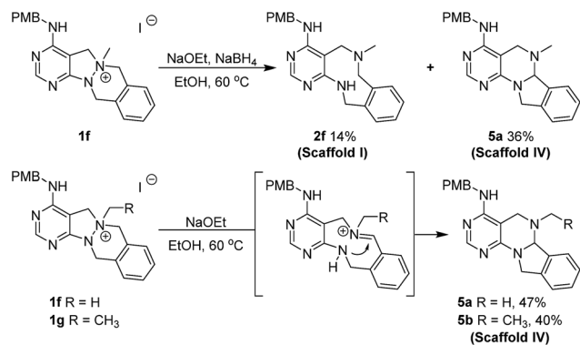
Scheme 3 Exploration of ring-rearrangement pathway (ii) for scaffold IV.
