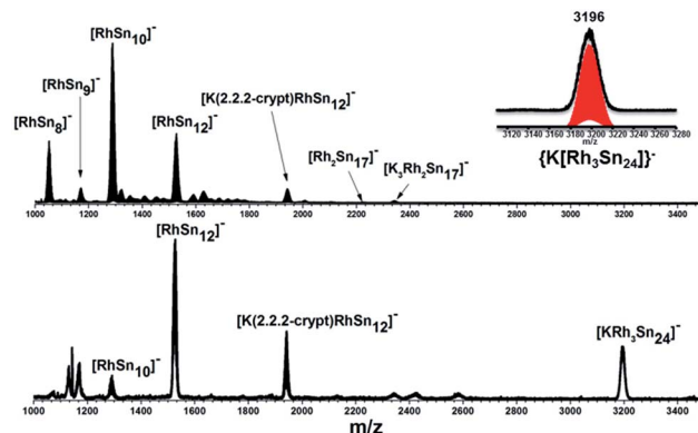
Fig. 1 ESI-MS ( m/z : 1000–3500) in negative ion mode of en(bottom) and DMF (up) reaction mixtures. The inset show the [\text{K}[\text{Rh}_3\text{Sn}_{24}]^-] peak and its simulated pattern.
