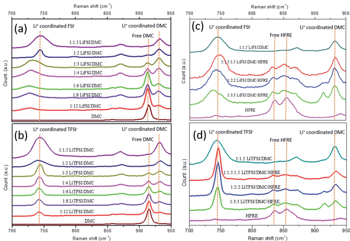
Fig. 1 Raman spectra of different electrolytes in the range of 700–950 \text{cm}^{-1} . (a) LiFSI/DMC electrolytes with different LiFSI/DMC molar ratios and pure DMC; (b) LiTFSI/DMC electrolytes with different LiTFSI/DMC molar ratios and pure DMC; (c) LiFSI/DMC/HFRE localized concentrated electrolytes with different molar ratios, highly concentrated LiFSI/DMC (molar ratio of 1:1.5) and pure HFRE; (d) LiTFSI/DMC/HFRE localized concentrated electrolytes with different molar ratios, highly concentrated LiTFSI/DMC (molar ratio of 1:1.5) and pure HFRE.
