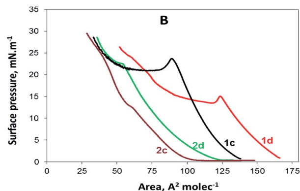
Fig. 2 (A) \pi - A isotherms of the gemini surfactants 1b , 1c and 1d containing benzyl ester groups and (B) \pi - A isotherms of all compounds ( 1c , 1d , 2c , and 2d ) having n = 8 and n = 12 .
