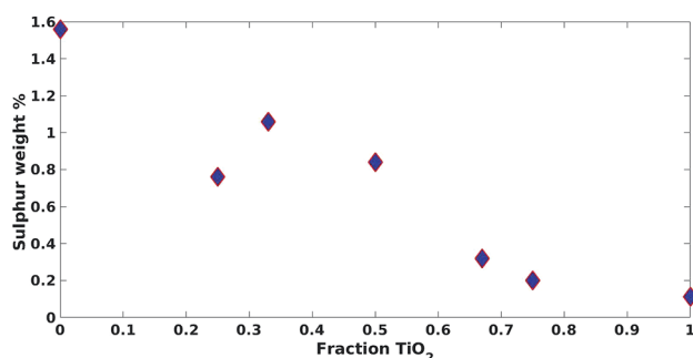
Fig. 9 Impact of increasing fraction of \text{TiO}_2 on approximated sulphur weight% from SEM/EDX.
