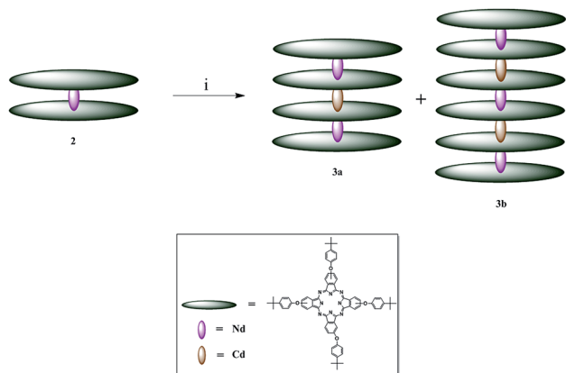
Scheme 1 Synthetic pathway to obtain complexes 3a and 3b ; i = \text{TCB} and cadmium acetate dihydrate at reflux temperature, 24 h.
