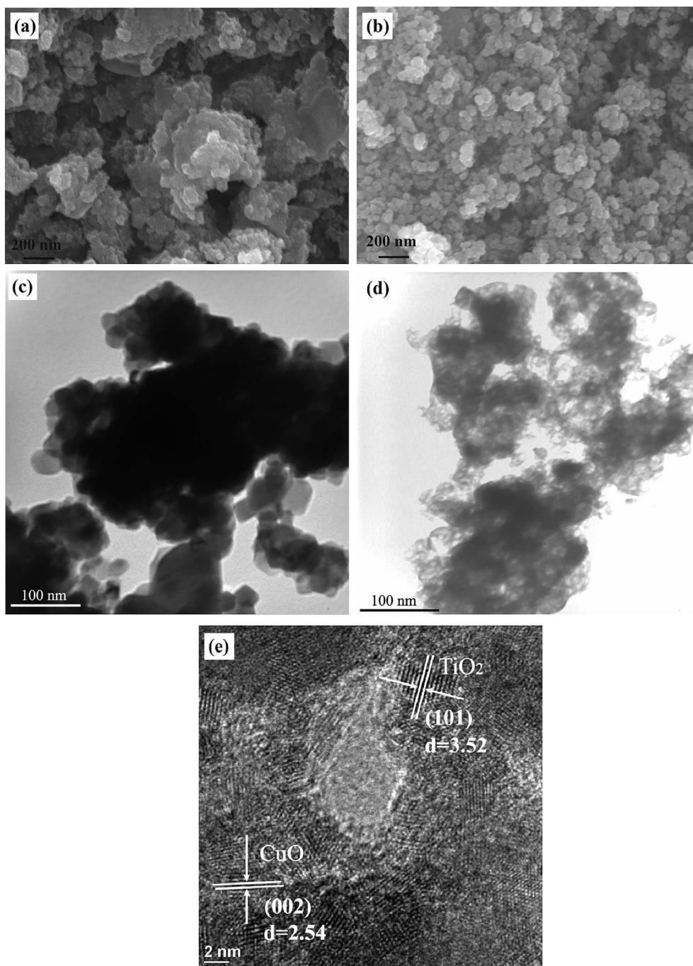
Fig. 4 SEM images of (a) TiO 2 and (b) CuO/TiO 2 , TEM images of (c) TiO 2 and (d) CuO/TiO 2 , and HR-TEM image (e) of CuO/TiO 2 catalyst.
