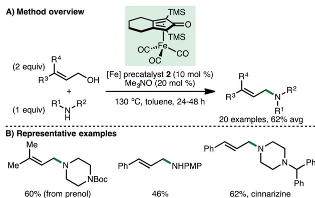
Scheme 6 Fe-Catalysed N -alkylation using allylic alcohols (Sundararaju).
