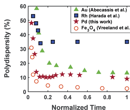
Fig. 3 Polydispersity as a function of normalized reaction time for Au (Abécassis et al. 39 (acidic ligand)), Rh (Harada et al. 46 (without NaCl)), Pd (our work), and Fe 3 O 4 (Vreeland et al. 27 ). Normalized time is defined as: time (experimental data collected)/time (end of reaction).
