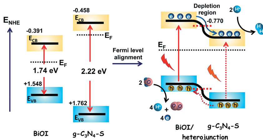
Fig. 8 Proposed mechanism of charge separation in g\text{-C}_3\text{N}_4\text{-S}/\text{BiOI} heterostructured photoanodes.
