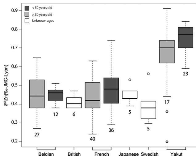
Fig. 6 Whisker plot of \delta^{66}\text{Zn} in the blood of various populations. The numbers below the boxes correspond to the sample size. The upper and lower limits of the boxes represent the 25th–75th percentiles (with the median as a bold horizontal line) and the whiskers show the 10th–90th percentiles. Data correspond to whole blood or erythrocyte values of populations from various geographical areas: Belgian individuals (whole blood); 10–12 Swedish individuals 3 (whole blood); Japanese individuals 4 (RBC), French individuals <50 years old 15 (RBC); Yakut individuals (whole blood), 14 and French individuals >50 years old (RBC) (this study, Supplementary Information 1, ESI†).
