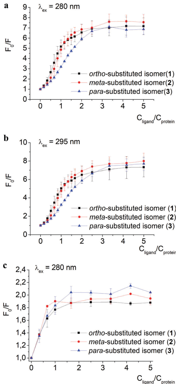
Fig. 2 Stern–Volmer plots of fluorescence intensity quenching of BSA emission excited at 280 (a) and 295 (b) nm, as well as of HSA emission excited at 280 nm (c), by clathrochelates 1–3 ; F_0 and F are protein fluorescence intensities in the absence and in the presence of these complexes. Spectra were recorded in 0.05 M Tris HCl, pH 7.9.
