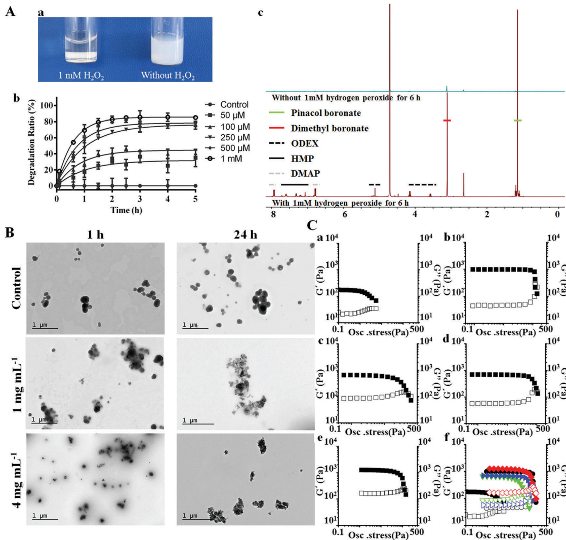
Fig. 2 (A) Investigation of the degradation of POD including (a) macroscopic images, showing H_2O_2 induced POD degradation; (b) quantitative investigation of degradation behavior via colorimetric method; (c) ^1H NMR spectrum of POD in D_2O with or without addition of H_2O_2 confirmed the degradation behavior of POD. (B) TEM images of D-G-PSi@POD with different concentrations of glucose at different time-points, suggesting the glucose dependent disassembly of the nanohybrid. (C) Mechanical characterization of different hydrogels showing the in situ nanoparticle/hydrogel transformation. Rheological dynamic oscillatory stress sweep tests of (a) C, (b) COD, (c) CP, (d) CP1, (e) CP4 and (f) the stacking figure. Solid data points in a–f correspond to the storage modulus G' . Open data points in a–f correspond to the loss modulus G'' . In f, black square, black circle, green down-triangle, blue right-triangle and red diamond respectively correspond to C, COD, CP, CP1 and CP4.
