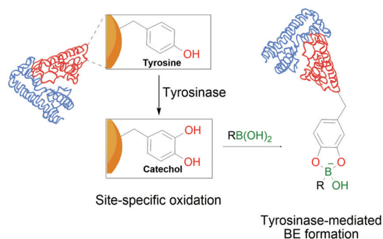
Fig. 11 Oxidation of a tyrosine residue by tyrosinase to the corresponding catechol enables the formation of transient BEs on the protein's surface.
