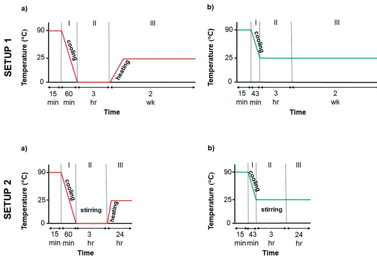
Fig. 2 Diagrams illustrate the different temperature profiles used in this study. Setup 1 is quiescent conditions and setup 2 is stirring conditions, each using controlled cooling to (a) 0 \text{ }^{\circ}\text{C} , and (b) 25 \text{ }^{\circ}\text{C} .
