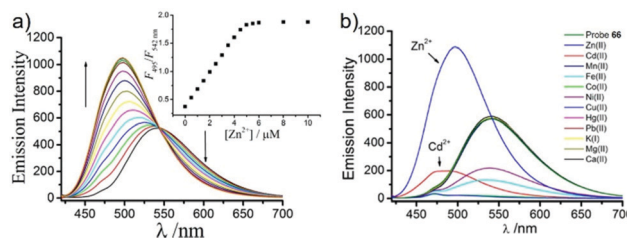
Fig. 110 (a) Fluorescence spectra of 5 μM 66 upon titration of Zn 2+ (0–10 μM) in aqueous buffer (20 mM MES, 0.1 M NaCl, pH = 5.2), \lambda_{\text{ex}} = 405 nm. Inset: The emission ratio ( F_{495}/F_{542\text{nm}} ) changes as a function of Zn 2+ concentration. (b) Fluorescence spectra of 66 (5 μM) in the presence of various metal ions (5 μM Mn 2+ , Fe 2+ , Co 2+ , Ni 2+ , Cu 2+ , Zn 2+ , Cd 2+ , and 1 mM Mg 2+ , Ca 2+ , and K + ) in MES buffer (pH = 5.2, \lambda_{\text{ex}} = 405 nm). Copyright 2012 American Chemical Society.
