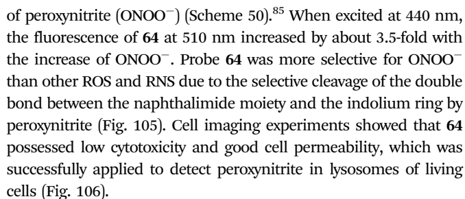
Scheme 50 Fluorescent probe 64 for ONOO - .
