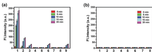
Fig. 108 (a) Time-dependent fluorescence response of 2 μM 65 to the testing species in HEPES buffer solution (10 mM, 0.5% DMSO, 0.5% TW 80, pH 5.0): 1, 10 μM AS; 2, 20 μM GSNO; 3, 200 μM ONOO - ; 4, 50 μM NOC-5; 5, 500 μM NO 2 - ; 6, 200 μM H 2 O 2 ; 7, 100 μM O 2 - ; 8, 20 μM MeLOOH; 9, 200 μM ClO - . (b) 1, 50 μM L-cys; 2, 100 μM GSH; 3, 500 μM NaHS; 4, 200 μM ascorbic acid; 5, 200 μM tocopherols; 6, 100 μM citrate; 7, 200 μM tyrosine (Tyr); 8, 50 μM hydroxylamine (HA). Bars represent fluorescence intensity during 0, 5, 10, 15, and 20 min after addition of various compounds. \lambda_{\text{ex}} = 690 nm, \lambda_{\text{em}} = 700 nm. Copyright 2014 Royal Society of Chemistry.
