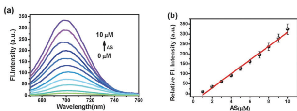
Fig. 107 (a) Fluorescence responses of 65 (2 μM) to different concentrations of Angel's salt (AS) with emission ranging from 670 to 760 nm. \lambda_{\text{ex}} = 690 nm. (b) Relationship between the relative fluorescence intensity at 700 nm and concentrations of AS (0, 1, 2, 3, 4, 5, 6, 7, 8, 9, 10 μM). Fluorescence spectra were acquired in HEPES buffer solution (10 mM, 0.5% DMSO, 0.5% TW 80, pH 5.0). Copyright 2014 Royal Society of Chemistry.
