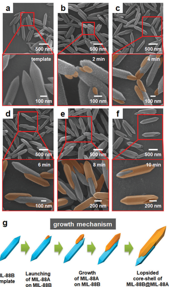
Fig. 2 SEM images monitoring the formation of the lopsided core-shell of MIL-88B@MIL-88A. The SEM images were acquired for the samples obtained from the reaction solution at different times (a) 0 min (initial template), (b) 2 min, (c) 4 min, (d) 6 min, (e) 8 min, and (f) 10 min. Newly grown MIL-88A portions are highlighted in orange in the magnified SEM images. (g) Mechanism for the unbalanced MOF-on-MOF growth of MIL-88A onto the MIL-88B template for the production of the lopsided core-shell of MIL-88B@MIL-88A.
