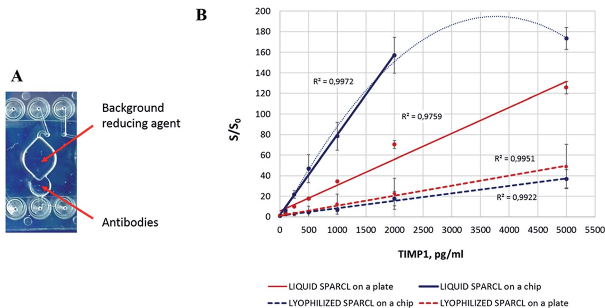
Fig. 4 The effect of the reagent lyophilization on the performance of the SPARCL™ assay. (A) Deposition of the lyophilized reagents on the chip. (B) Assay performance with liquid and lyophilized reagents (number of replicates n = 3 ).
