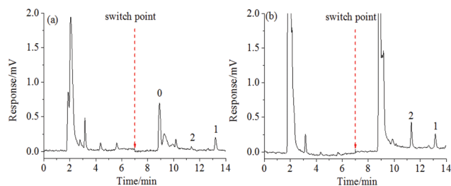
Fig. 6 Nonspecific adsorption of OTA on the PMAA monolith (a) and PEA monolith (b) peak 0: background compound, peak 1: ochratoxin A, peak 2: ochratoxin B. The concentrations of OTA and OTB were 0.2 \text{ ng mL}^{-1} and 10 \text{ ng mL}^{-1} , respectively.
