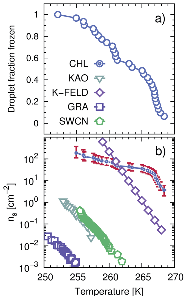
Fig. 1 CHLM crystals promote the formation of ice across a wide range of temperatures. (a) Droplet fraction frozen as a function of temperature for 1\ \mu\text{m} water droplets placed onto a CHLM substrate. (b) Ice-active surface site density n_s (see text and Methods section) values for the same data reported for CHLM (CHL) in panel (a), together with n_s values for kaolinite (KAO) from Herbert et al. , 62 BCS376 feldspar (K-FELD) from Atkinson et al. , 11 graphene oxide (GRA) from Whale et al. 63 and single-walled carbon nanotubes (SWCN) also from ref. 63. The uncertainty in terms of temperature associated with the CHLM data is \pm 0.4 K.
