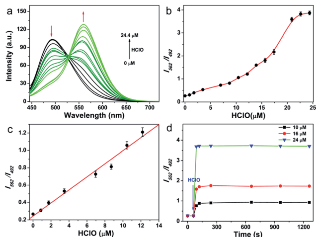
Fig. 1 (a) Fluorescence spectra of 5.0 μM QC10 upon the addition of HClO (0–24.4 μM). (b) Plot of the fluorescence intensity ratio (562 nm/492 nm) change of 5.0 μM QC10 versus HClO − concentration (0–24.4 μM). (c) Linear relationship between the fluorescence intensity ratio and HClO concentration in the range of 0.8–12.5 μM. (d) Plot of the fluorescence intensity ratio of QC10 as a function of HClO (10, 16, and 24 μM). The excitation wavelength was 426 nm in 10 mM PBS (pH = 7.4, containing 5% DMF) buffer solution.
