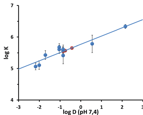
Fig. 5 Plot of the \log K vs. \log D (pH = 7.4) values relative to the binding of the luminescent analytes 8 – 13 and 17 – 19 to S1-AuNP. The lines represent the linear fit of the data ( R = 0.885 ). Red circles report the affinity values estimated for substrates 1 , 14 and 15 on the basis of their \log D values and the fitting parameters. The error bars reported represent the confidence intervals ( 3\sigma ) calculated from standard deviations reported in Table 1.
