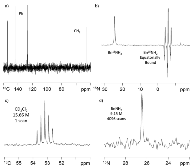
Fig. 3 (a) ^1\text{H} - ^{13}\text{C} refocused INEPT NMR spectrum of hyperpolarised \text{BnNH}_2 (35 mM) achieved via 2\text{-BnNH}_2 (5 mM) under SABRE in dichloromethane- d_2 solution after transfer at 60 G and 308 K; (b) ^{15}\text{N} NMR spectrum of ^{15}\text{N} -labelled \text{Bn}^{15}\text{NH}_2 (35 mM) after SABRE transfer via 2\text{-BnNH}_2 (5 mM) at 60 G and 308 K which gives rise to hyperpolarised resonances for free ( \delta 24.42) and equatorially bound ( \delta -5.59 ) substrate; (c) single scan thermally polarised ^{13}\text{C} NMR spectrum in \text{CD}_2\text{Cl}_2 (15.66 M) and (d) 4096 scan thermally polarised ^{15}\text{N} NMR spectrum of \text{BnNH}_2 (9.15 M).
