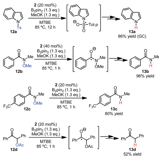
Scheme 11 Reductive cleavage reactions employing the diboron/MeOK/2 system.
