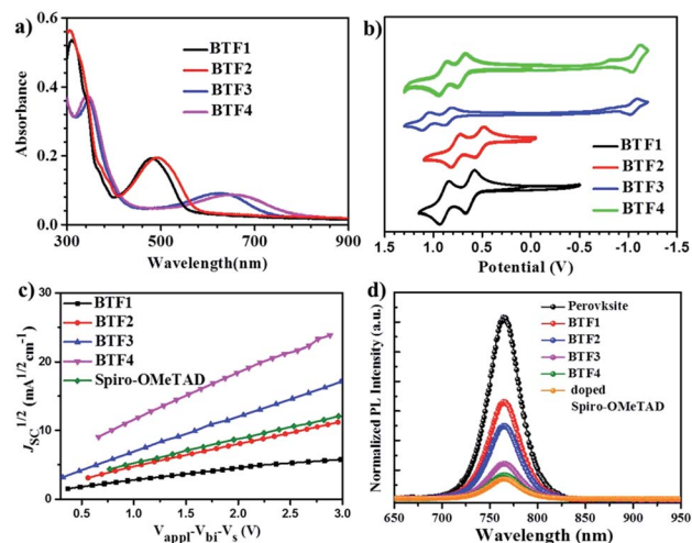
Fig. 2 (a) The film absorption spectra. (b) The CV curves versus \text{Fe}/\text{Fe}^{+} (0.66 V) measured in DCM solution. (c) The hole injection characteristics measured by the SCLC method based on the device structure of \text{ITO}/\text{V}_2\text{O}_5/\text{HTMs}/\text{V}_2\text{O}_5/\text{Al} . (d) Steady state PL spectra of the bilayered perovskite films with or without capping with different HTLs.
