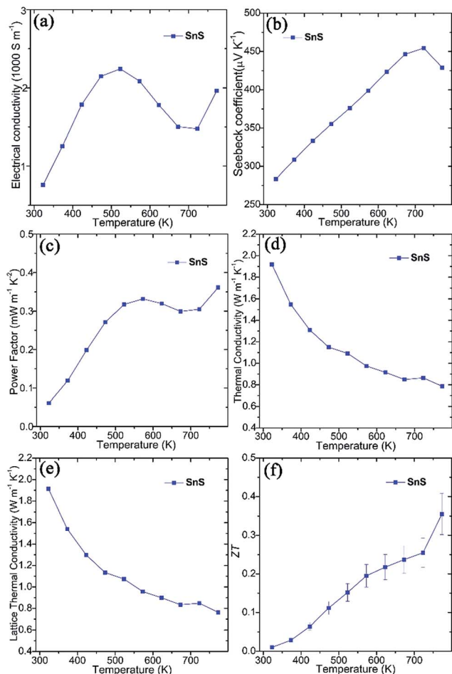
Fig. 2 Thermolectric properties of SnS pellets sintered using SPS, measured perpendicular to the pressing direction: (a) the electrical conductivity ( \sigma ), (b) the Seebeck coefficient ( S ), (c) the power factor ( S^2\sigma ), (d) the thermal conductivity ( \kappa ), (e) the lattice \kappa ( \kappa_L ), and (f) ZT as a function of temperature.
