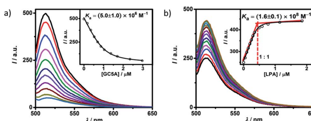
Fig. 1 (a) Direct fluorescence titration of FI (1.0 μM) with GC5A (up to 3.0 μM), λ ex = 500 nm. (Inset) the associated titration curve at λ em = 513 nm and the fit according to a 1 : 1 binding stoichiometry. (b) Competitive titration of GC5A·FI (0.4/0.5 μM) with LPA (up to 1.9 μM). (Inset) fit of the titration data to a 1 : 1 competitive binding model. All experiments are in HEPES buffer (10 mM, pH = 7.4) at 25 °C.
