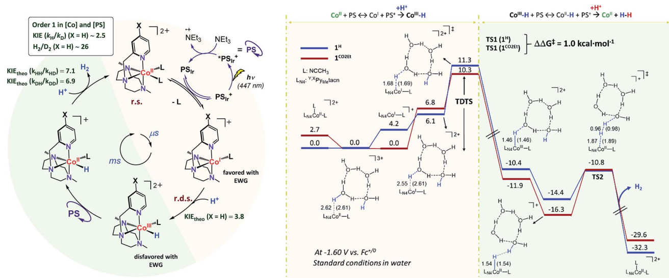
Fig. 11 (Left) Proposed mechanism for \text{H}_2 evolution catalysed by 1^{\text{R}} complexes. (Right) values are \Delta G . Energies are given in \text{kcal mol}^{-1} . B3LYP- \text{D}_3/\text{aug-cc-pVTZ}(-\text{f})//\text{B3LYP-}\text{D}_3/6-31+\text{G}^* level of theory. Bond lengths for 1^{\text{H}} ( 1^{\text{CO}_2\text{Et}} ) are shown in Årmstrongs.
