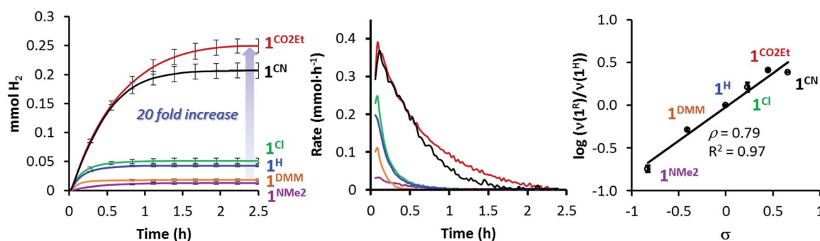
Fig. 4 On-line traces and rates of \text{H}_2 formed vs. time for \mathbf{1}^{\text{R}} complexes (Left and Middle, respectively). Conditions: \mathbf{1}^{\text{R}} (50 \mu\text{M} ) and \text{PSIr}^+ (150 \mu\text{M} ) in \text{CH}_3\text{CN} : \text{H}_2\text{O} : \text{Et}_3\text{N} (4 : 6:0.2 mL) irradiated ( \lambda = 447 \text{ nm} ) at 25 °C. (Right) Hammett plot of \log(\nu(\mathbf{1}^{\text{R}})/\nu(\mathbf{1}^{\text{H}})) (at 10% conversion) vs. the \sigma Hammett value. \mathbf{1}^{\text{CN}} (black), \mathbf{1}^{\text{CO}_2\text{Et}} (red), \mathbf{1}^{\text{Cl}} (green), \mathbf{1}^{\text{H}} (blue), \mathbf{1}^{\text{DMM}} (orange) and \mathbf{1}^{\text{NMe}_2} (purple).
