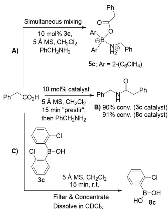
Scheme 6 Examining bis-2-chlorophenylboronic acid 3c as a catalyst for direct amide formation and ^{11}\text{B} NMR spectra of product mixtures obtained in 3 examined cases.
